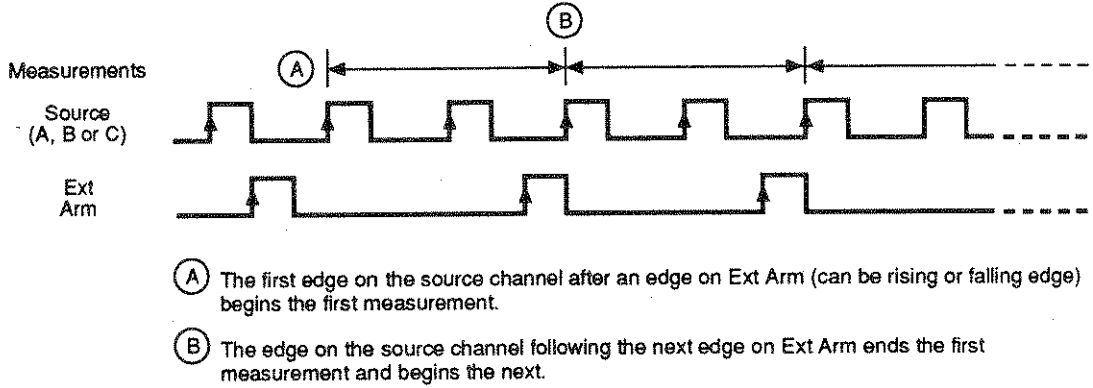
Figure 9-2. Frequency with Ext Arm Sampling
