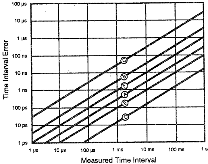
Graph 4 Time Interval Reference Error. Crystal aging will affect your Time Interval accuracy.
