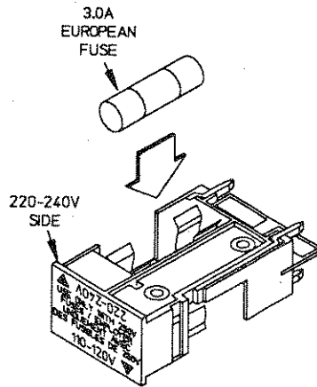
(a) CHECKING AND INSTALLING EUROPEAN FUSE
