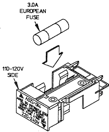
(a) CHECKING AND INSTALLING EUROPEAN FUSE
