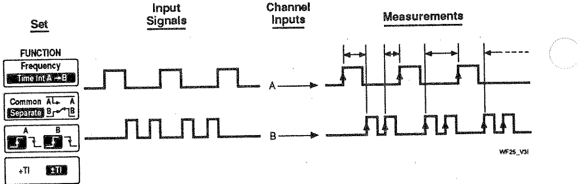
Figure 2-5. \pm TI A→B with Separate Inputs
