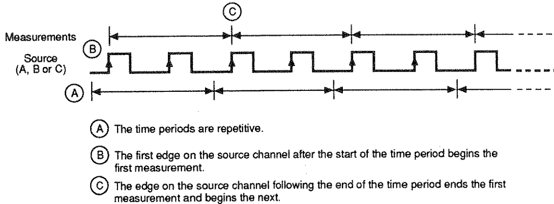
Figure 9-3. Frequency with Time Sampling
