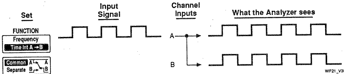
Figure 2-1. Time Interval A→B with Common Inputs
