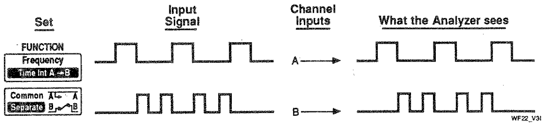
Figure 2-2. Time Interval A→B with Separate Inputs
