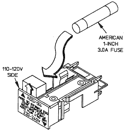
(b) CHECKING AND INSTALLING AMERICAN FUSE
